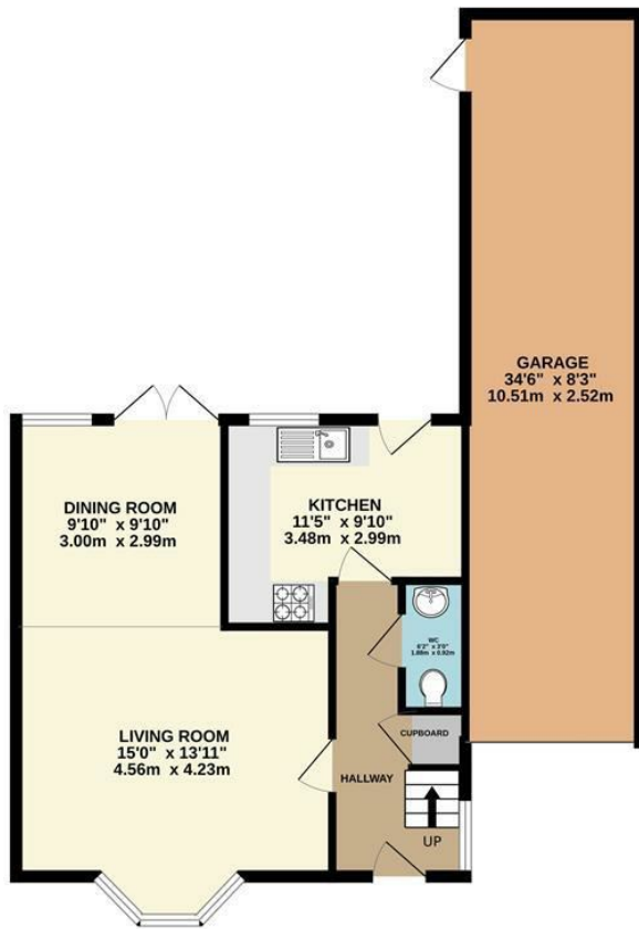
GROUND FLOOR 755 sq.ft. (70.1 sq.m.) approx.
